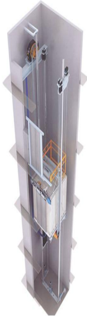
Machine roomless elevator
